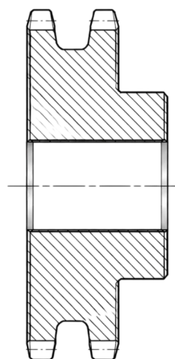
Double row sprocket for heavy duty applications.
