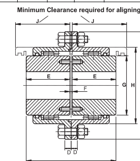
Couplings Size 101 To 110
