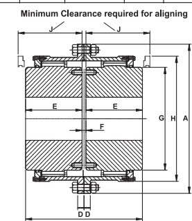
Couplings Size 111 To 119
