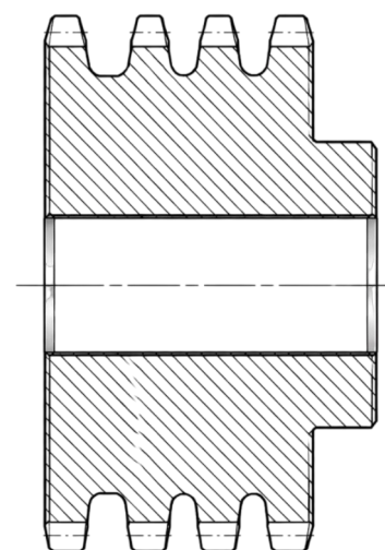
Triple row sprocket for extra heavy duty applications.
