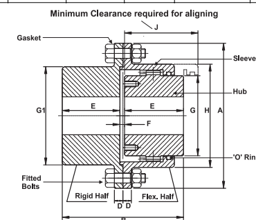
Half Flexible Couplings
